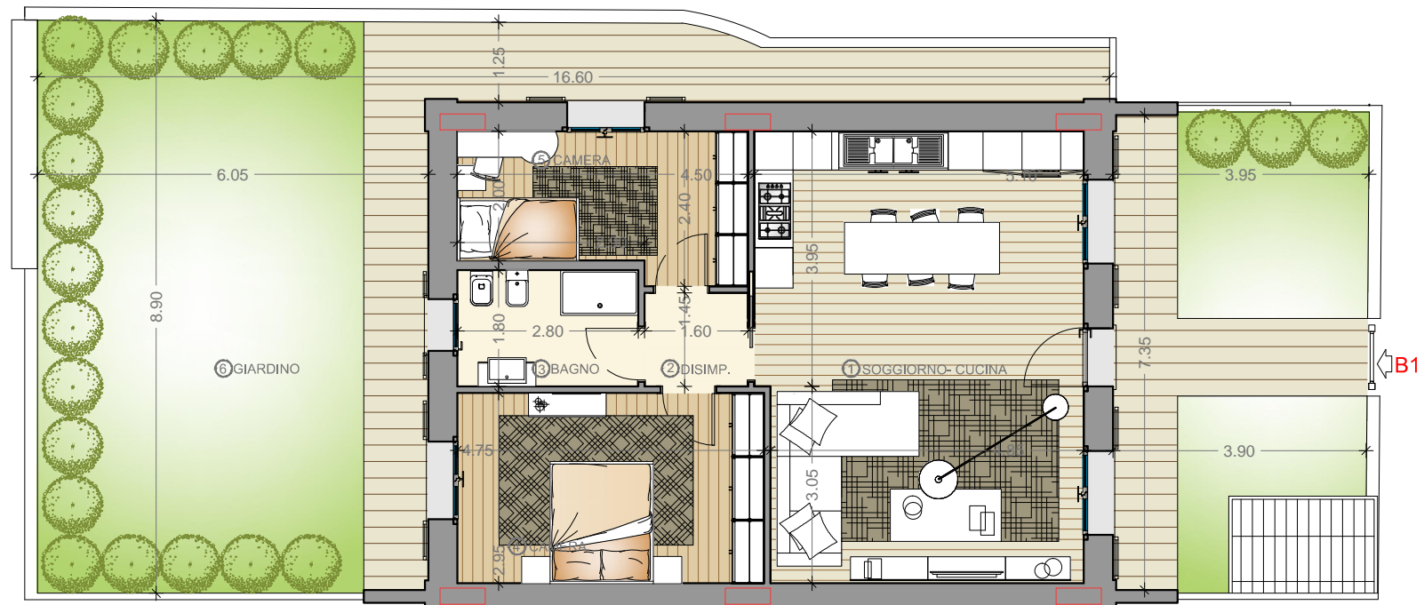
PLANIMETRIA PIANO TERRA
