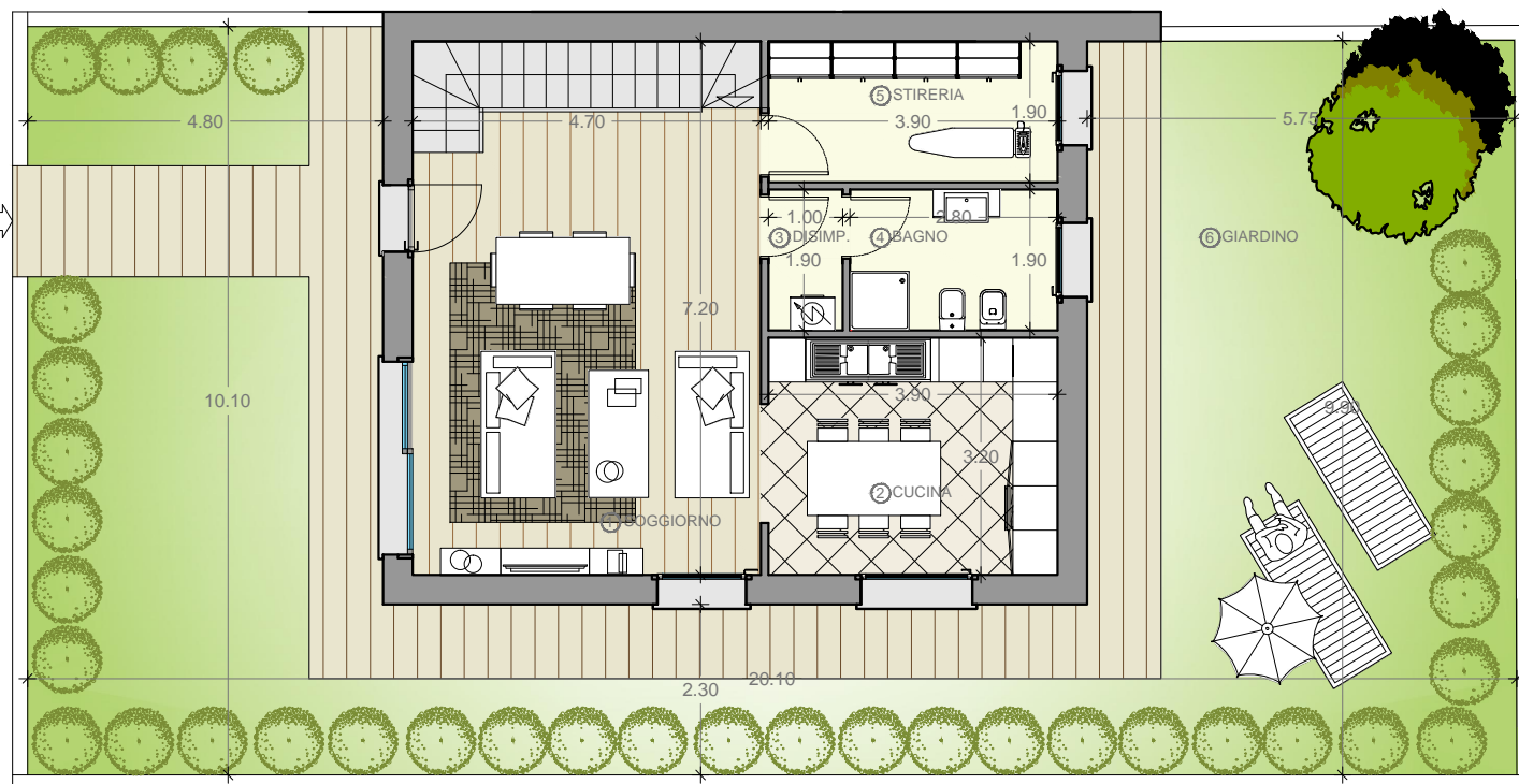
PLANIMETRIA PIANO TERRA
