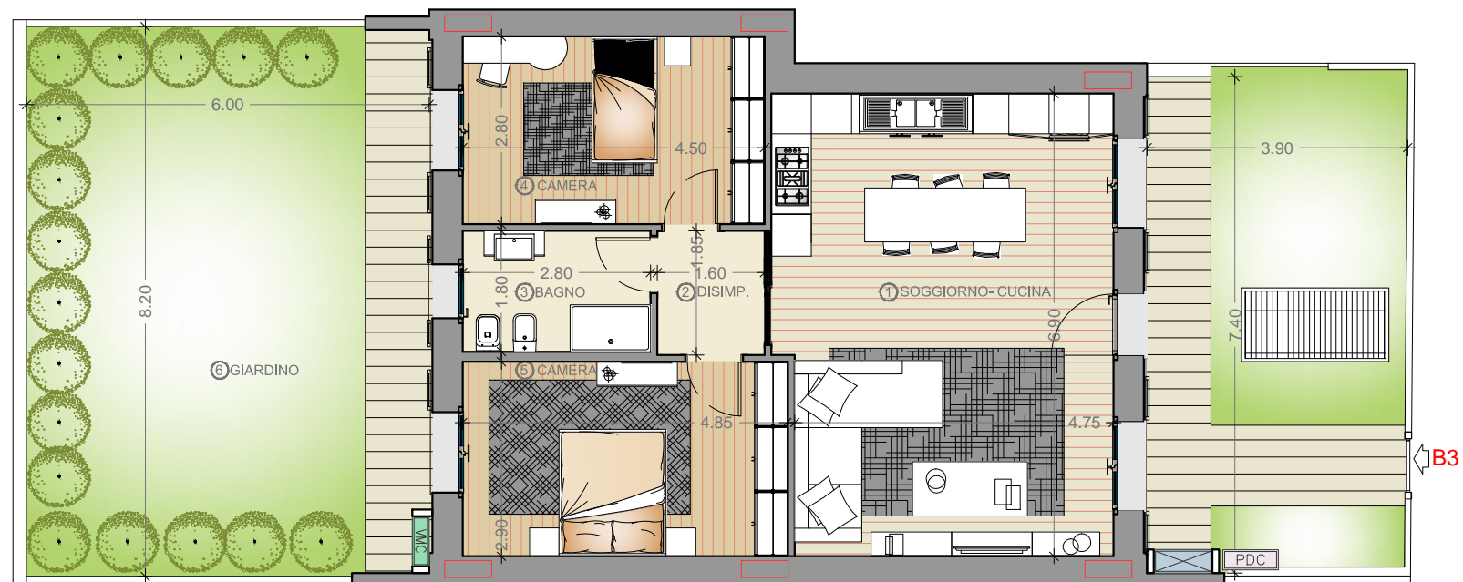
PLANIMETRIA PIANO TERRA
